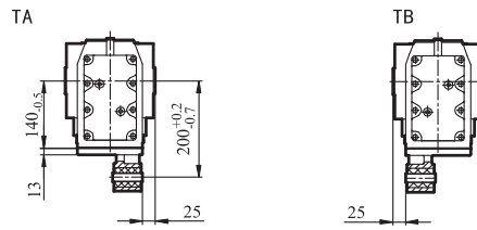
GKH/GKHZ/GKHF67输出轴
