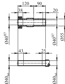
GKH/GKHZ/GKHF67输出轴
